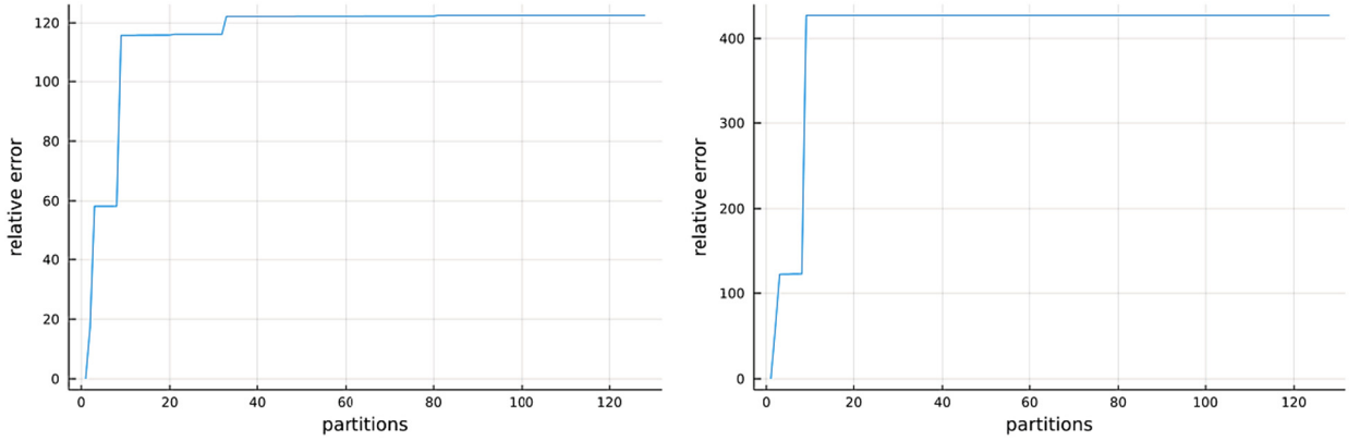
Fig. 6. Maximum relative error for 128 different partitions, sorted in ascending order. Left: initial states \mathcal{X}_0 . Right: initial states \mathcal{X}_0^L .
